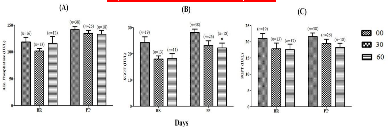
Graph 1. Effect of BR and PP on Liver function parameters
